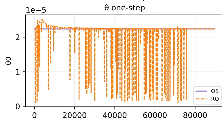
Oracle theta fit — sample 366
