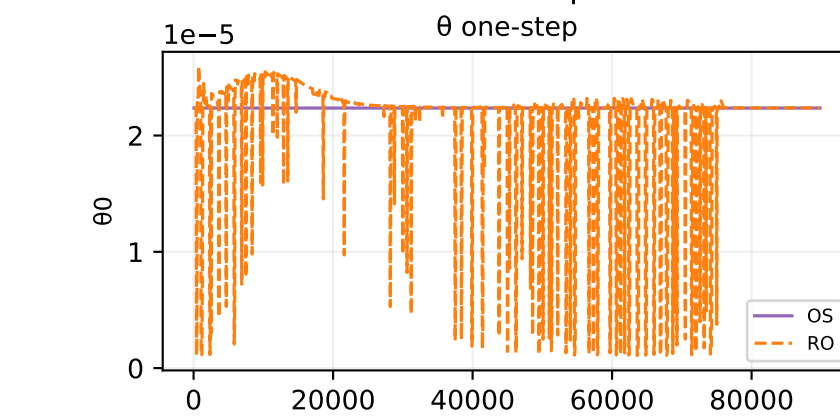
Oracle theta fit — sample 369
