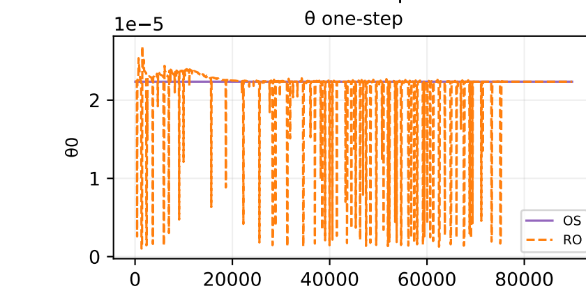
Oracle theta fit — sample 380
