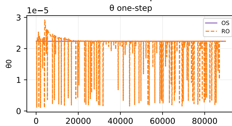
Oracle theta fit — sample 393
