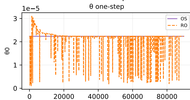
Oracle theta fit — sample 396
