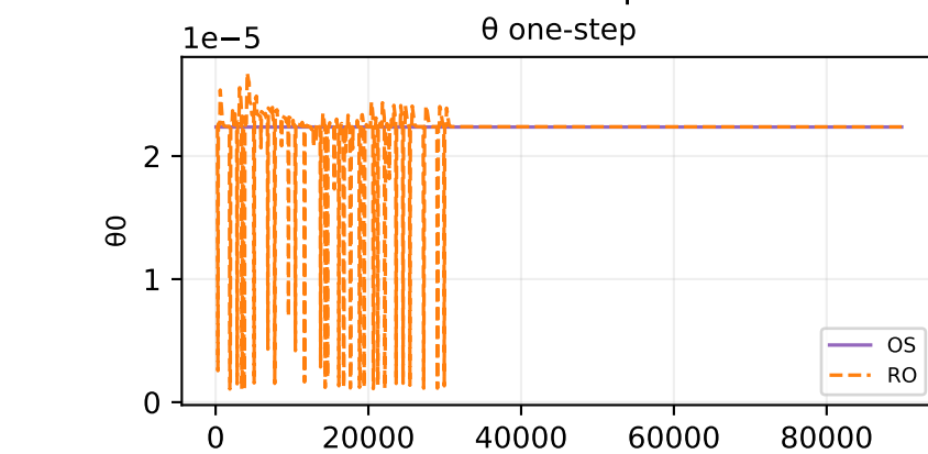
Oracle theta fit — sample 399
