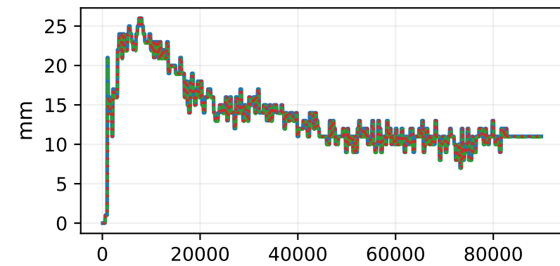
\theta_4
