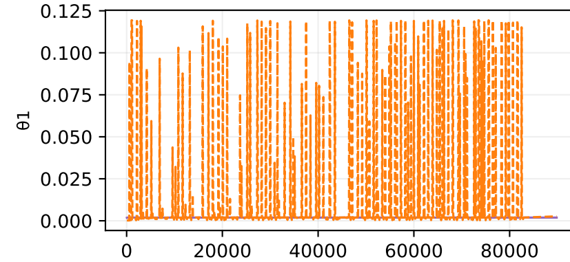
\theta rollout
