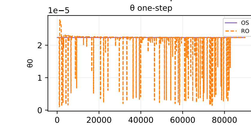
Oracle theta fit — sample 427
