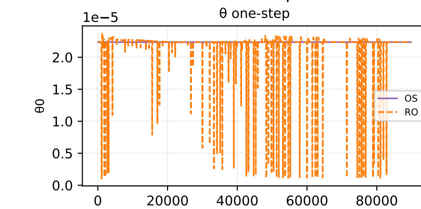
Oracle theta fit — sample 428
