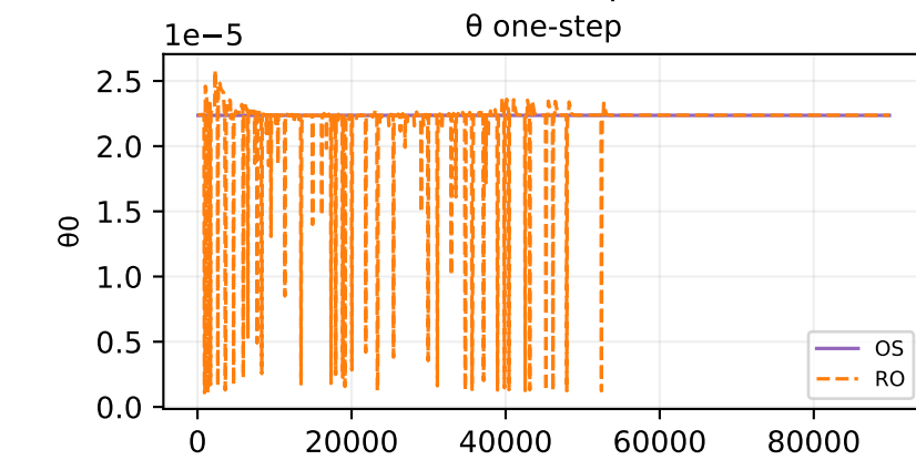
Oracle theta fit — sample 442
