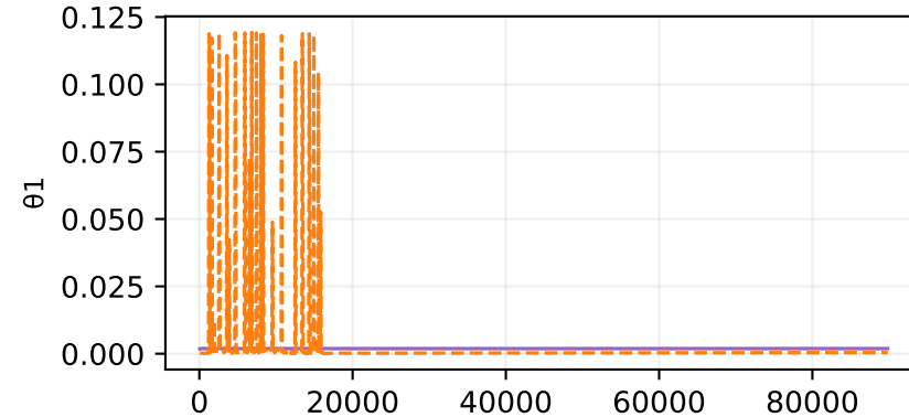
\theta rollout
