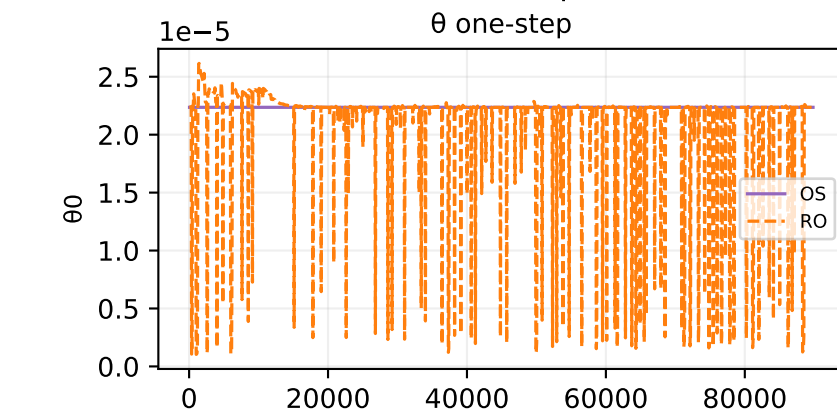
Oracle theta fit — sample 456
