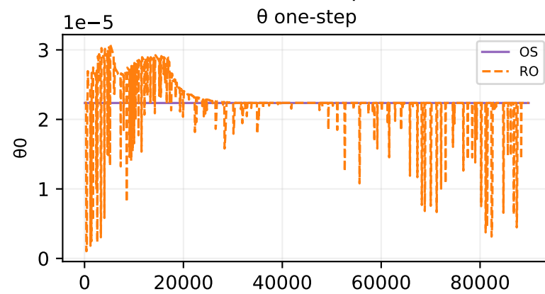
Oracle theta fit — sample 467
