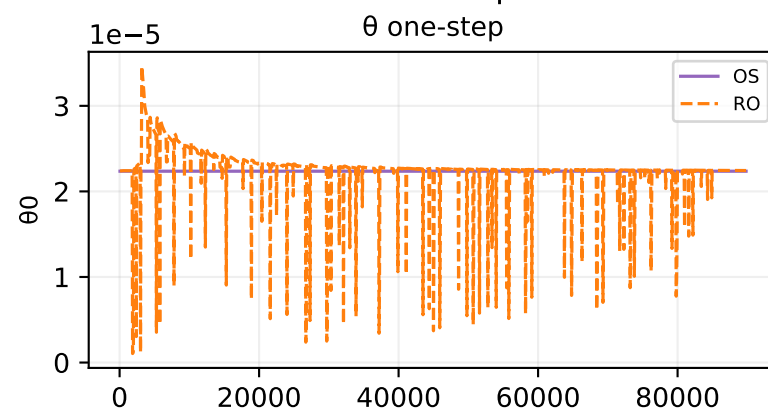
Oracle theta fit — sample 485
