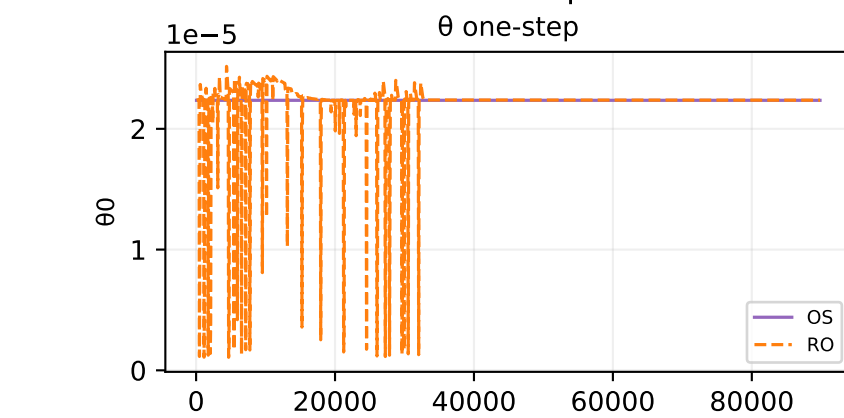
Oracle theta fit — sample 507
