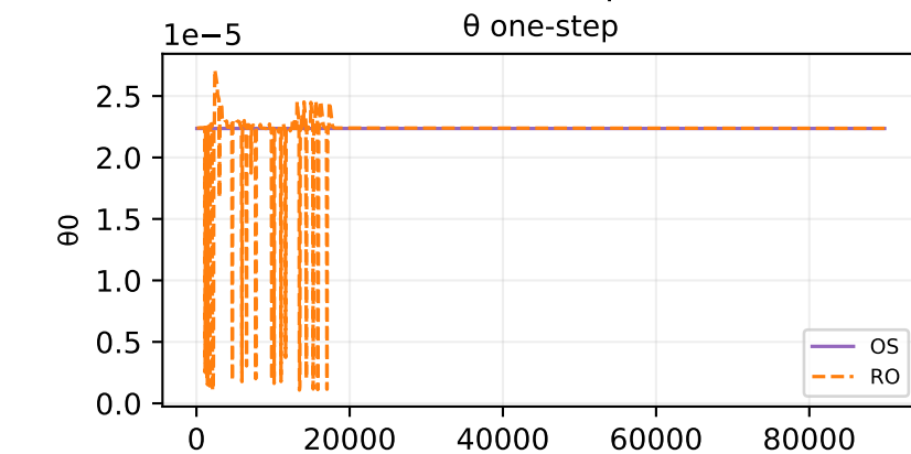
Oracle theta fit — sample 520
