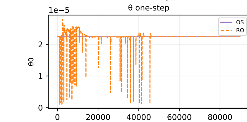
Oracle theta fit — sample 524
