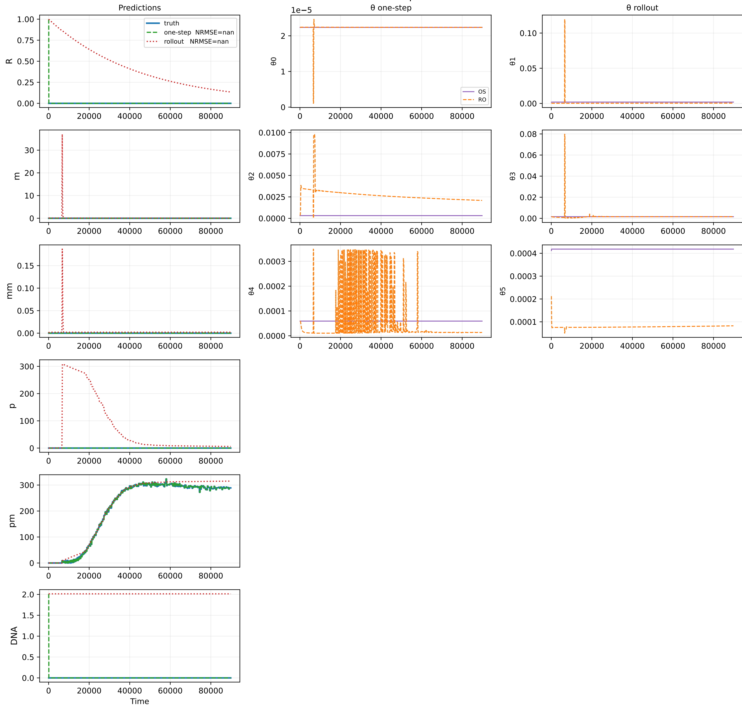
Oracle theta fit — sample 552
