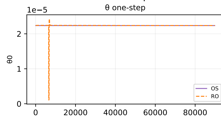
Oracle theta fit — sample 556
