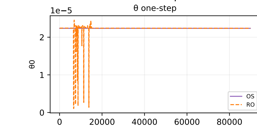
Oracle theta fit — sample 571
