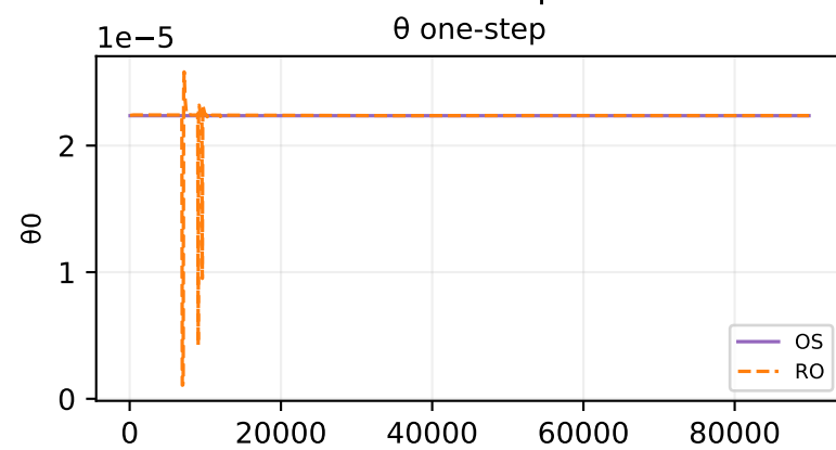
Oracle theta fit — sample 593
