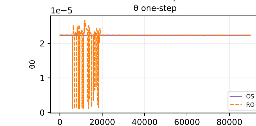
Oracle theta fit — sample 599
