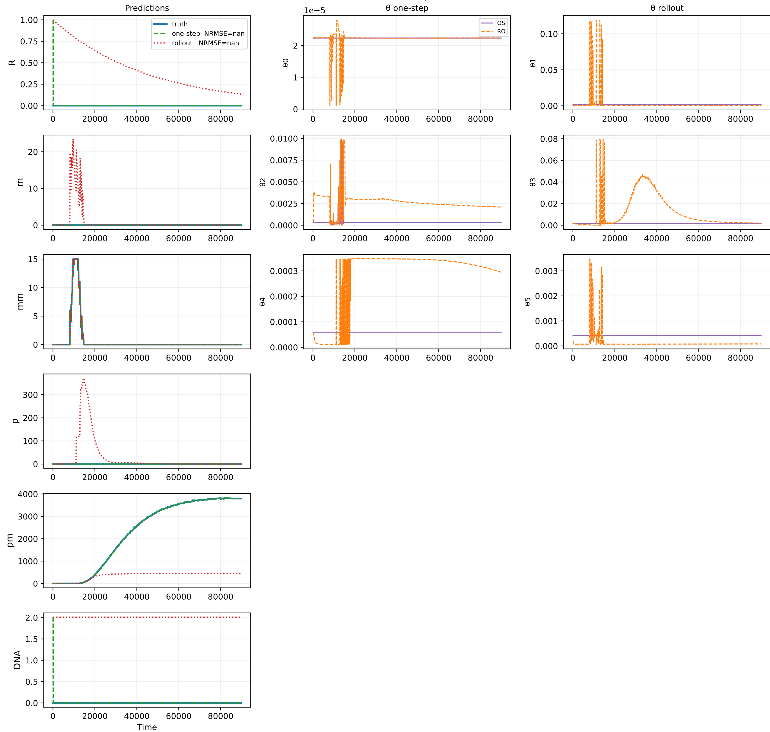
Oracle theta fit — sample 602
