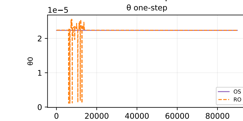
Oracle theta fit — sample 627
