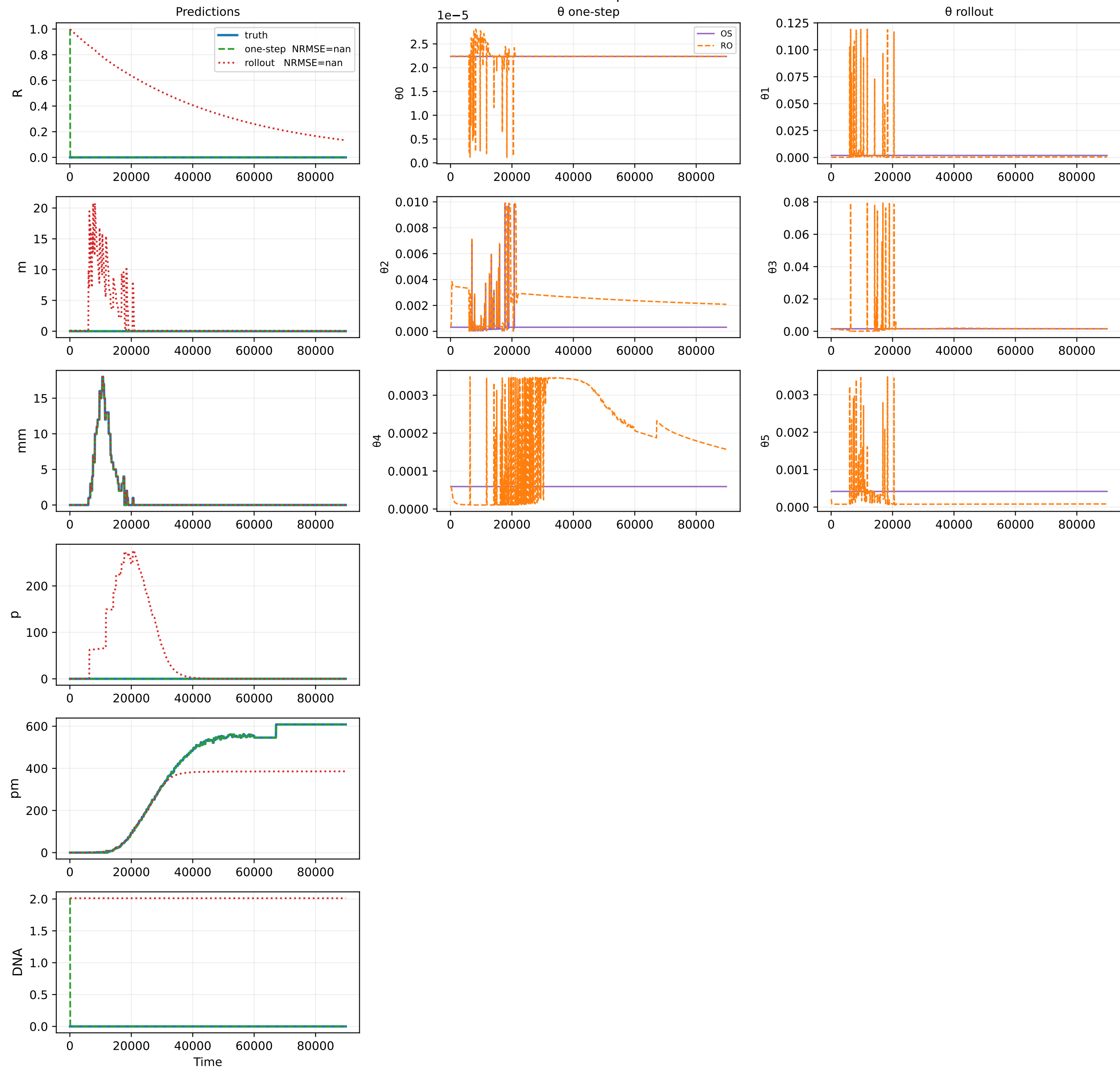
Oracle theta fit — sample 631
