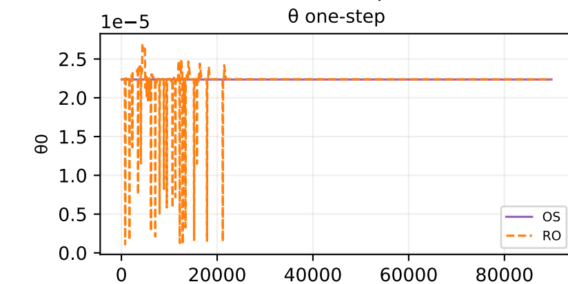
Oracle theta fit — sample 674
