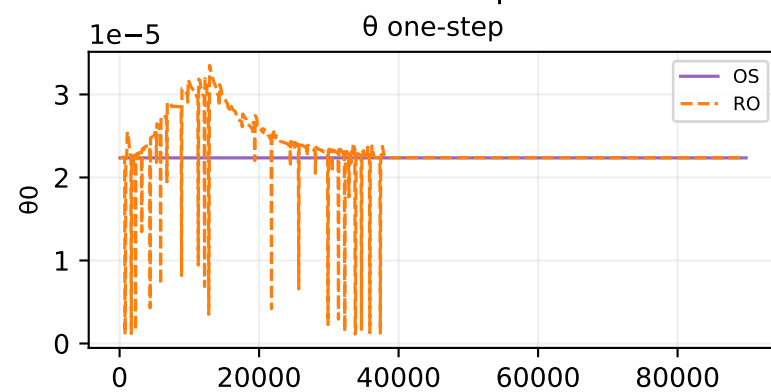
Oracle theta fit — sample 682
