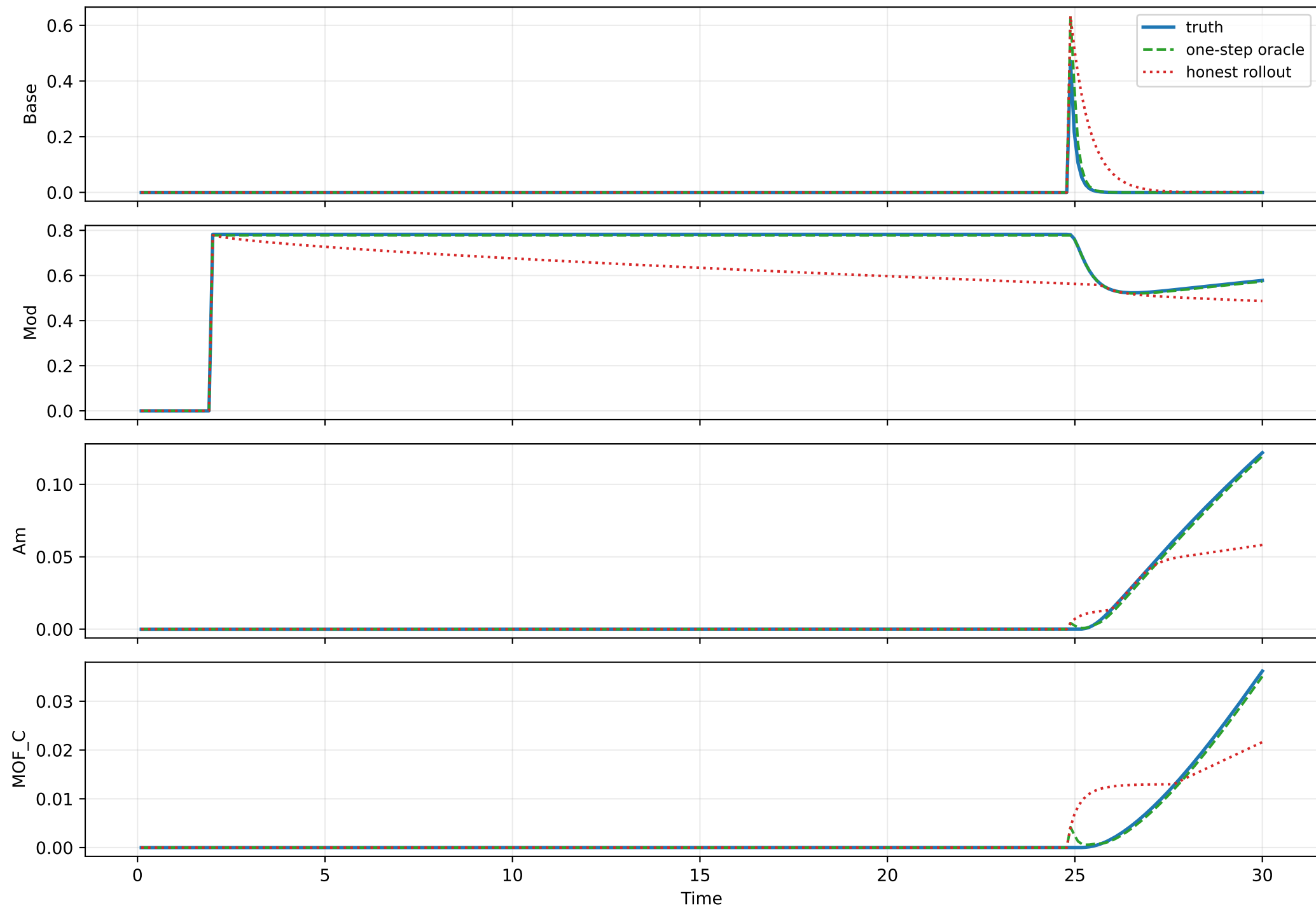
Oracle theta fit — mof_synthesis_4 (P=4) sample 0
