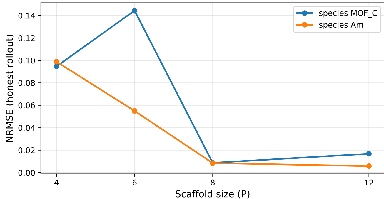
Trajectory error vs mechanistic scaffold size
