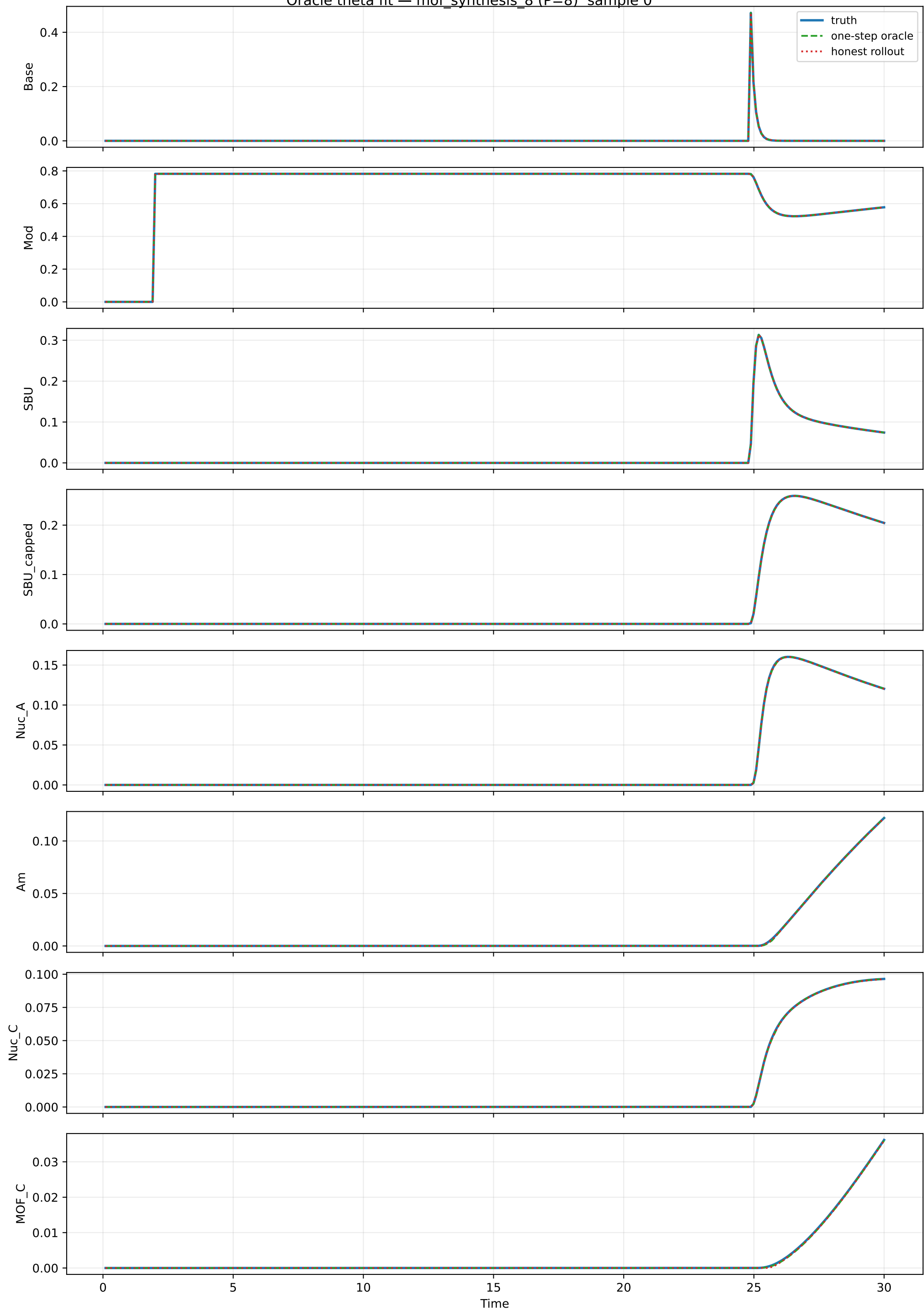
Oracle theta fit — mof_synthesis_8 (P=8) sample 0
