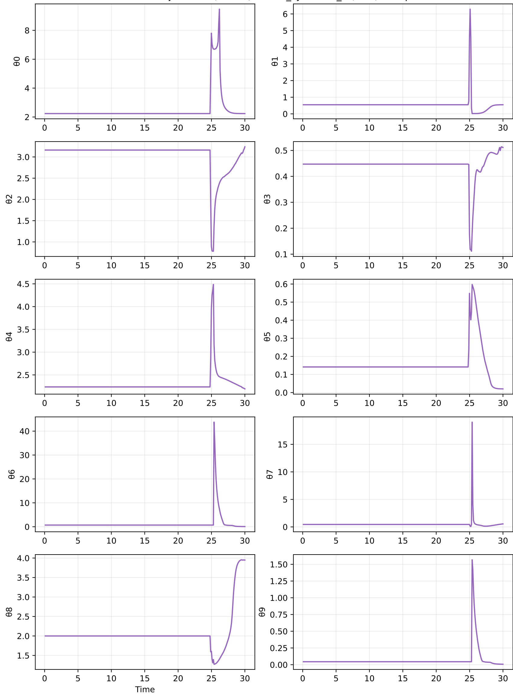
Oracle theta trajectories (rollout) — mof_synthesis_6 (P=6) sample 0
