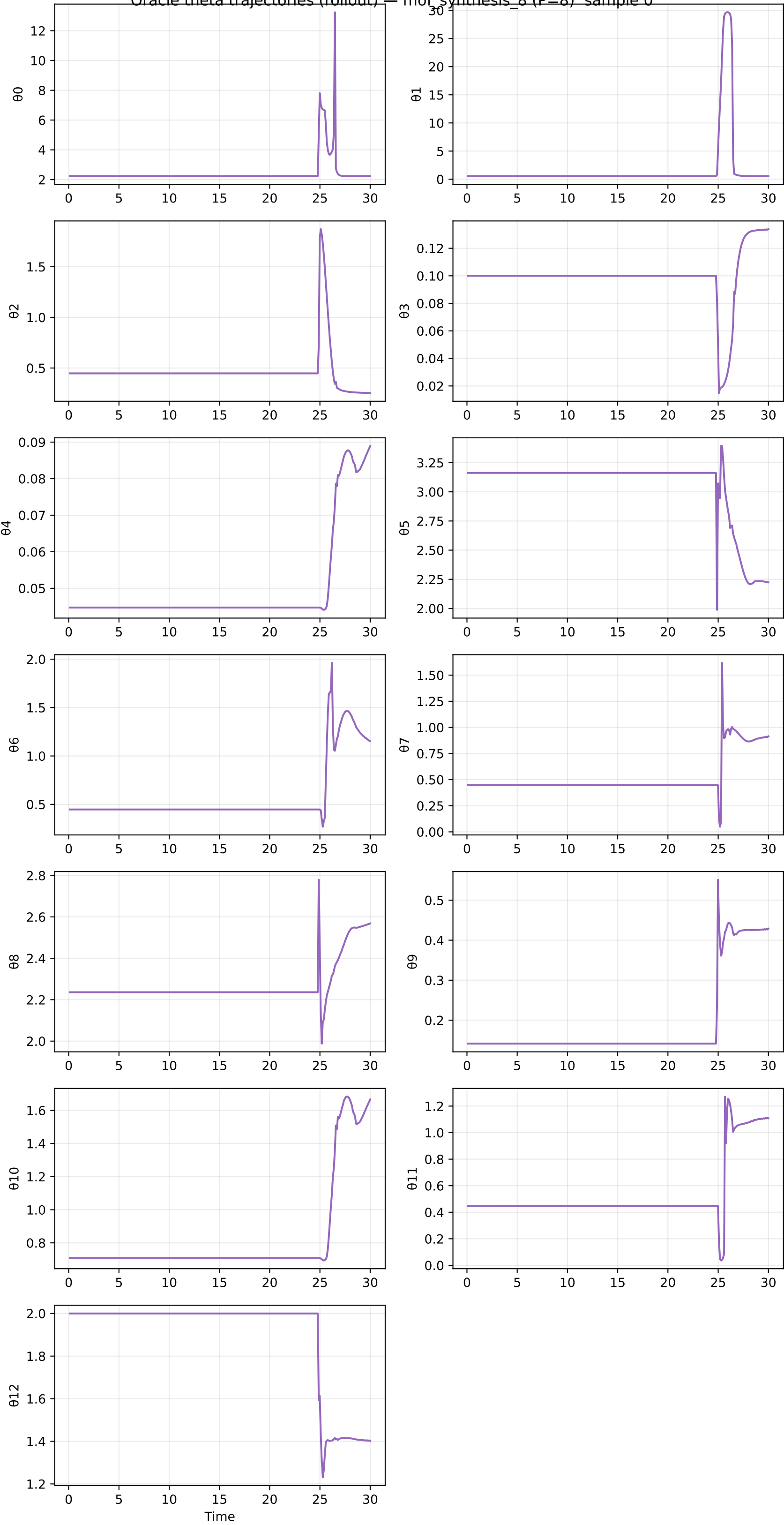
Oracle theta trajectories (rollout) — mof_synthesis_8 (P=8) sample 0
