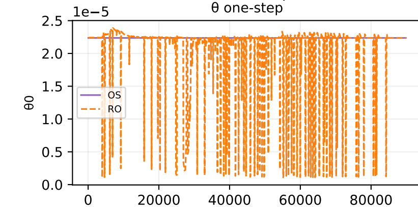
Oracle theta fit — sample 29
