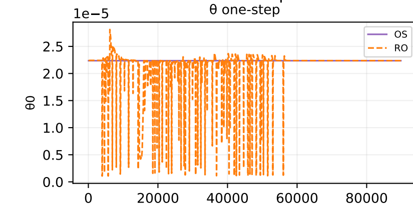
Oracle theta fit — sample 39
