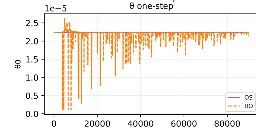
Oracle theta fit — sample 85
