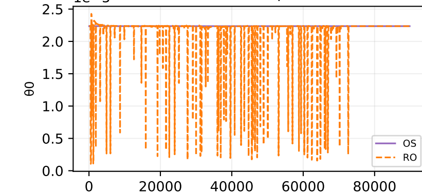
Oracle theta fit — sample 169
