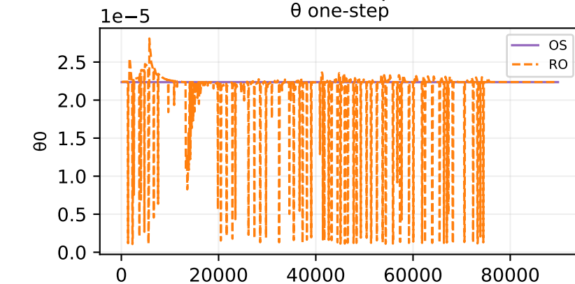
Oracle theta fit — sample 205
