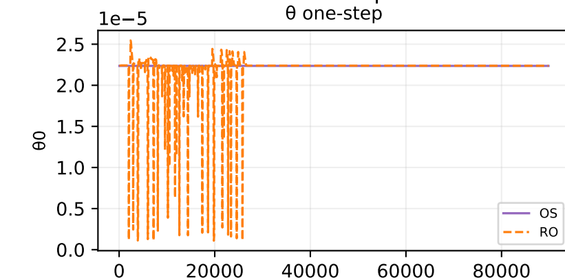
Oracle theta fit — sample 231
