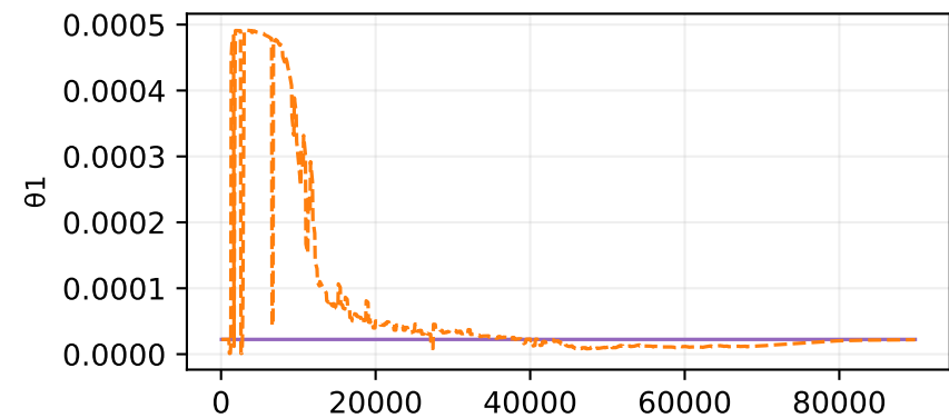
\theta rollout
