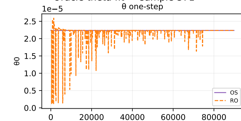
Oracle theta fit — sample 371
