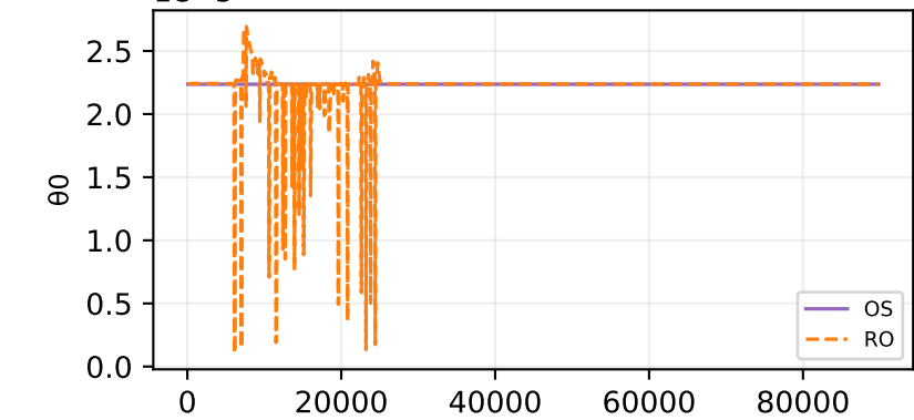
Oracle theta fit — sample 670
