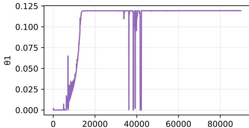
Oracle theta trajectories (rollout) — txtl_maturation_dna (P=6) sample 0
