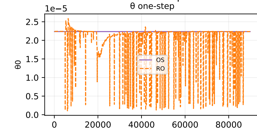
Oracle theta fit — sample 4
