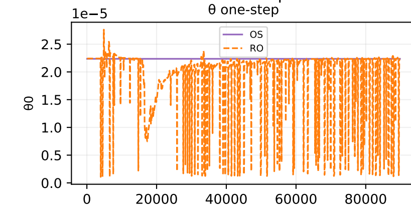
Oracle theta fit — sample 73
