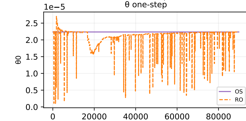
Oracle theta fit — sample 121
