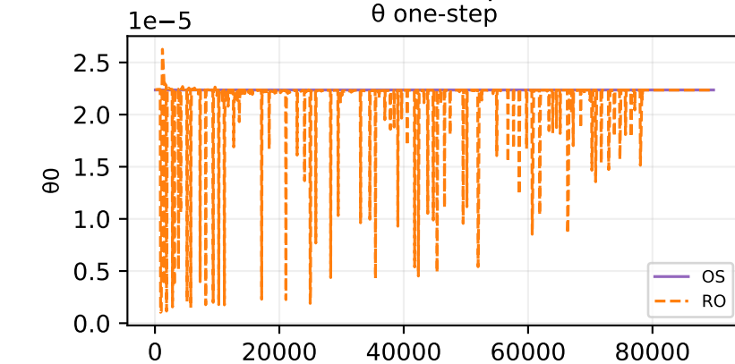
Oracle theta fit — sample 159
