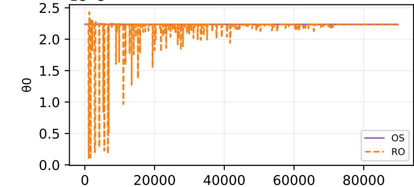
Oracle theta fit — sample 257 \theta one-step
