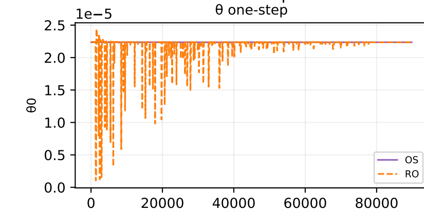
Oracle theta fit — sample 282
