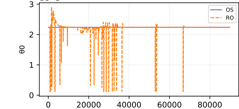
Oracle theta fit — sample 307 θ one-step
