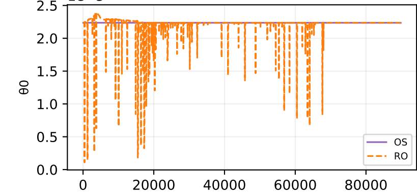
Oracle theta fit — sample 359 θ one-step
